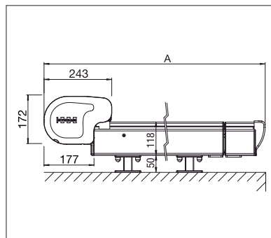
PS6100 Vista lateral
